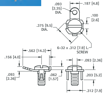
Mounting Detail
